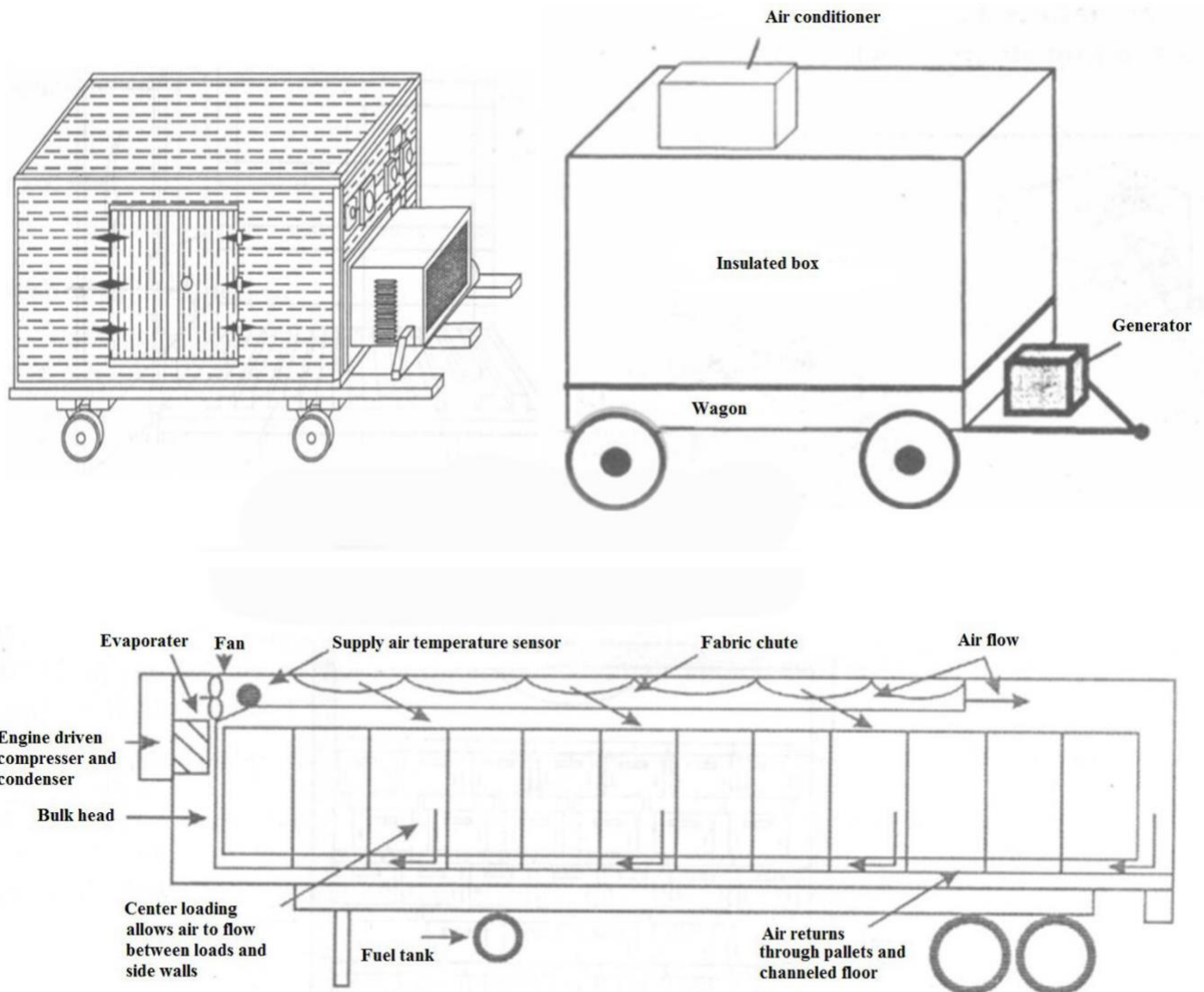
Fig. Refrigerated road transport vehicles
