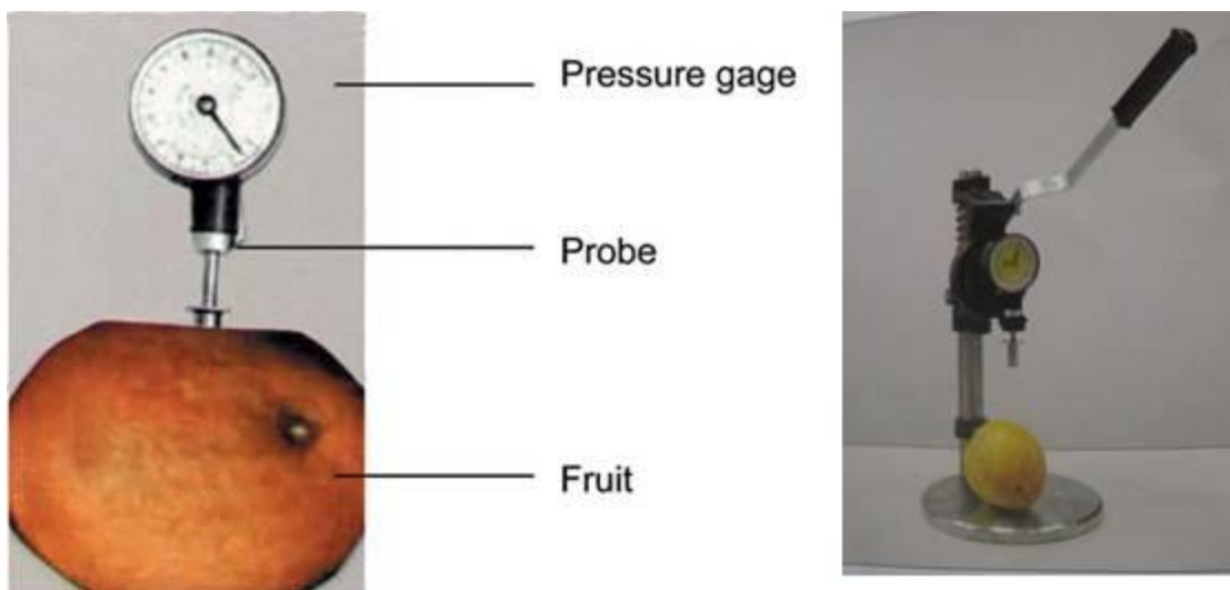
Fig. Objective firmness measurement using Penetrometer
