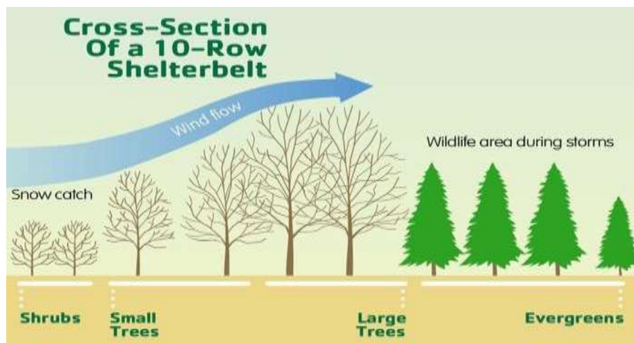
Fig. 3.5 A cross section of 10-row shelterbelts
