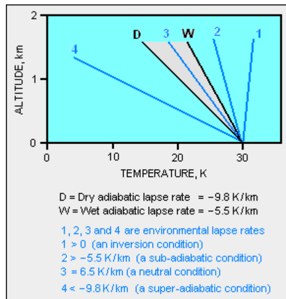
Fig.16 : Dry and saturated adiabatic lapse rate
