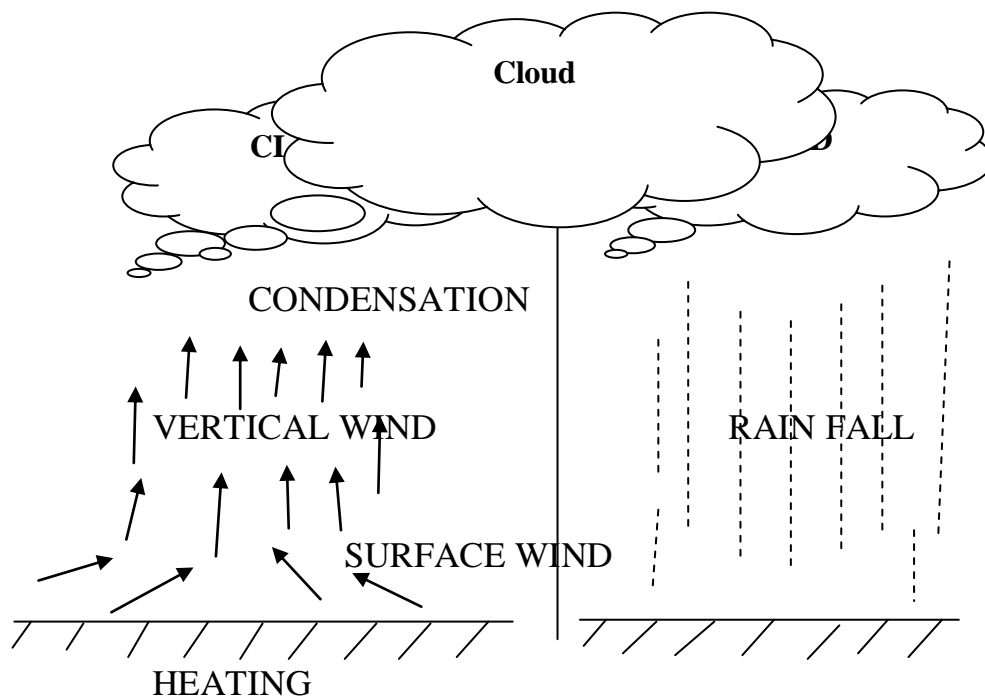
Fig.20 : Convective precipitation
