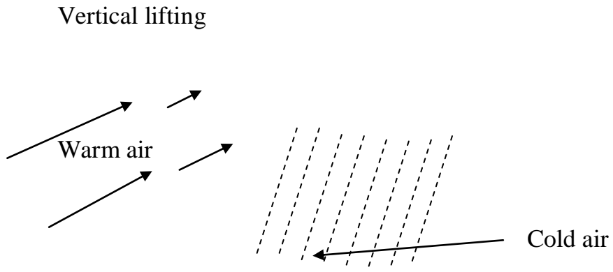
Fig.21 : Cyclonic or frontal precipitation
