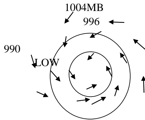
Fig.10: Cyclone
