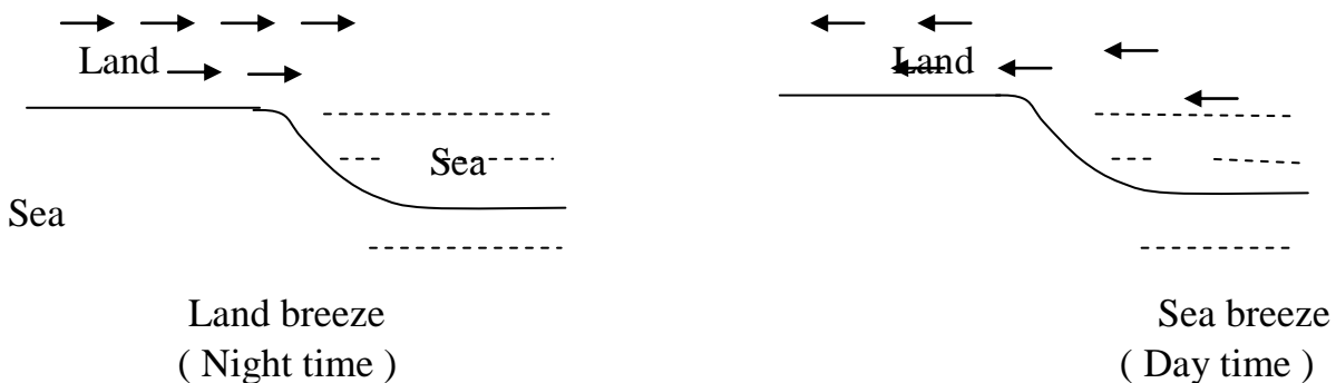
Fig.6 : Land and sea breeze
